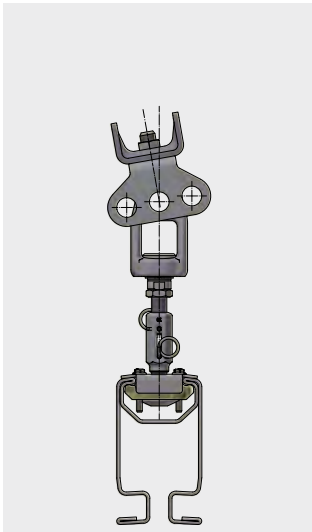
Inclined suspension
