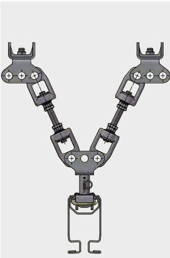
V-suspension
