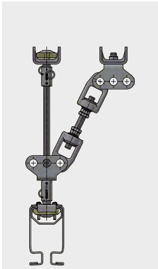
Standard stiffener
