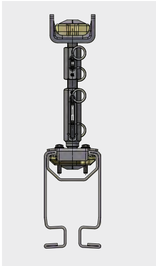
Normal suspension
