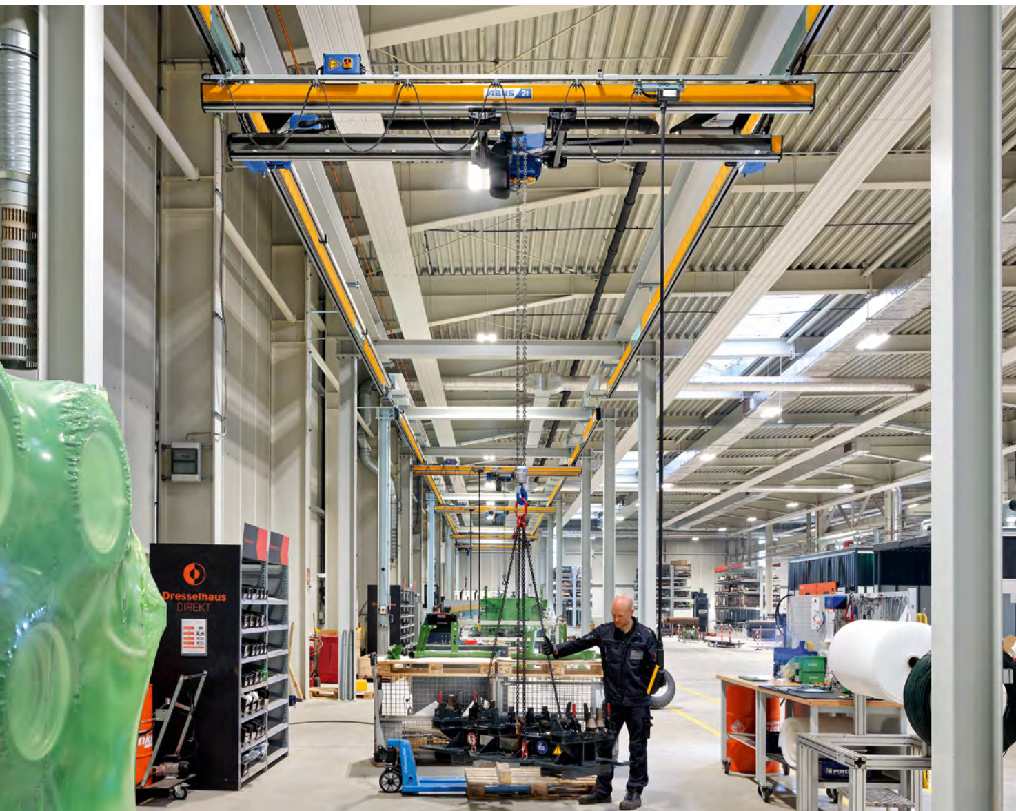
Fitted to rolled section I-beam using clamps
