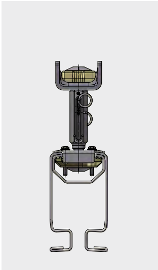
Short suspension
